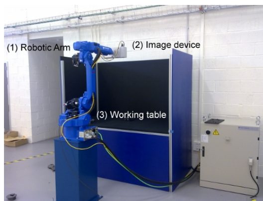
Fig. 2. The architecture of the machine vision system. (1) is the robotic arm of the system, (2) is the image device of the system and (3) is the working table where the castings are put for analysis.
